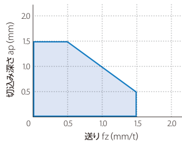
MFH40...
