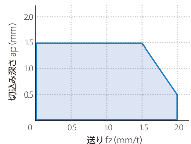
MFH40...
