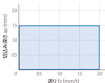
MFH050... ~ MFH080...
